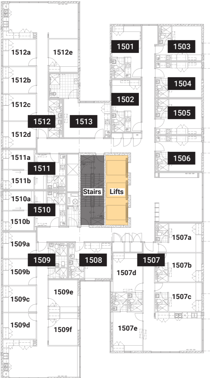
LEVEL 15 FLOOR PLAN
